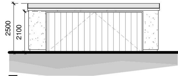
East. 1 : 100
